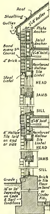
Wall Section
